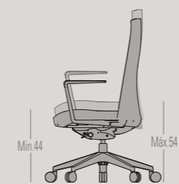
SEAT HEIGHT ADJUSTMENT. GAS LIFT Lowest seat height: 44 cm Maximum seat height: 54 cm
