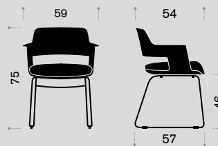
Sled base stationary chair Silla fija varilla Chaise fixe tube plein
